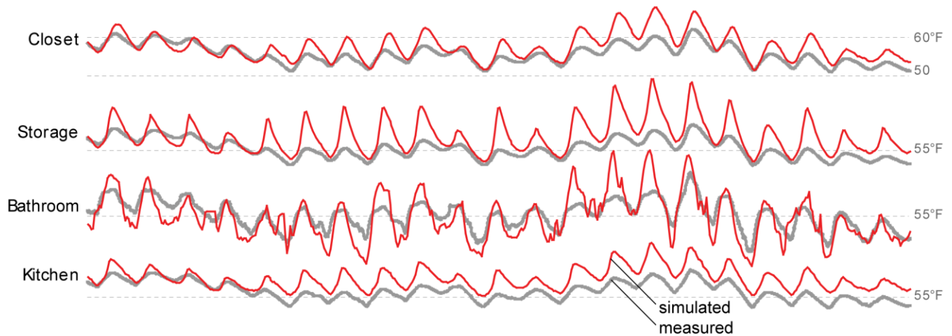
Figure 5. Before calibration: time series visualization of simulated and measured zone air temperatures for first 3 weeks of monitoring period.
