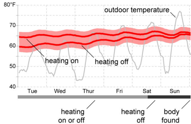
Figure 7. Projected temperature variation in the downstairs closet during the time period of interest.
