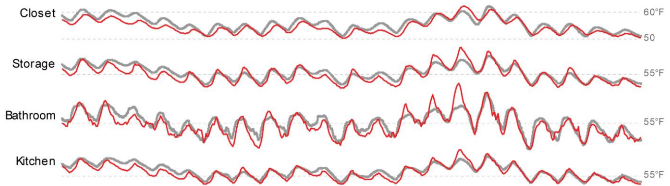
Figure 6. After calibration: time series visualization of simulated and measured zone air temperatures for first 3 weeks of monitoring period.
