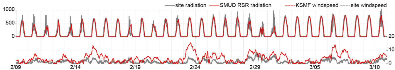
Figure 4. Comparison of solar radiation (left axis, W/m 2 ) and wind speed (right axis, mph) between local and site weather stations.
