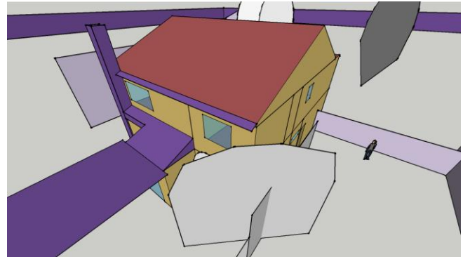
Figure 3. Screen capture of the energy model geometry. Note that two-dimensional purple and white objects are providing shade, while orange and red objects define thermal zones.
